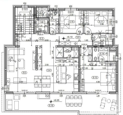
2.Stock/2.kat
