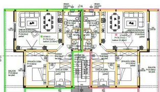
GRUNDRISS 1. STOCK
