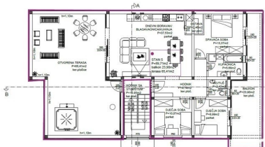
GRUNDRISS 2. STOCK
